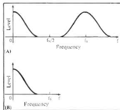
Figure 3. Spectrum of sampled audio signal of Figure 1 (lower sampling rate) as represented at the D/A (top curve—A) and as represented in the digital domain (bottom curve—B).
