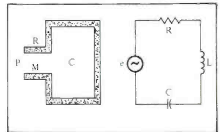
Figure 1. The acoustic and electrical analogs of a Helmholtz resonator.
